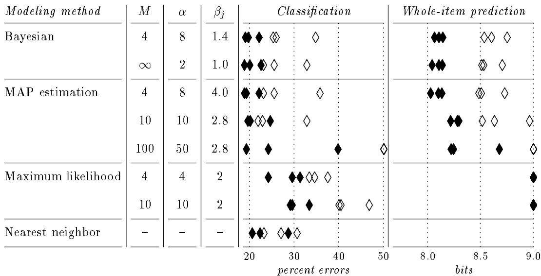
Figure 7: Comparative performance of Bayesian prediction, MAP estimation, maximum likelihood estimation, and nearest neighbor classification. Results on the small training sets are plotted with “ \diamond ”; those on the large training sets with “ \blacklozenge ”.
