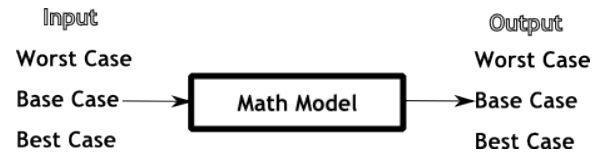
Figure 2: Case-based modeling.
